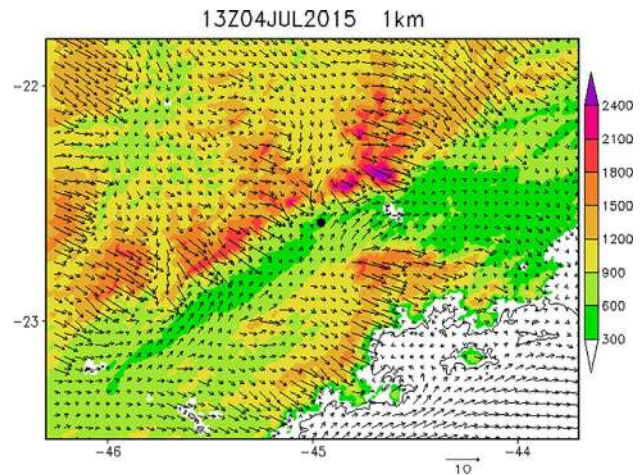
Figure 9 - Surface wind (in \text{m s}^{-1} ) as simulated by the Eta-1 valid for 4 July 2015 at 13 UTC (1-h simulation) and terrain elevation as seen by the model (colors bar in meters above sea level). The black dot indicates the location of Cruzeiro City.
