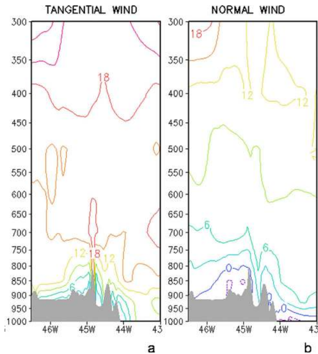
Figure 7 - As in Fig. 6 but for the wind component parallel (a) and perpendicular (b) (in \text{m s}^{-1} ) to the transect. Positive values are northwesterly wind in panel a, and southwesterly wind in panel b.
