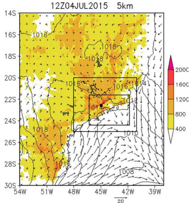
Figure 4 - Sea level pressure (contours in hPa) and surface wind ( \text{m s}^{-1} ) as simulated by the Eta-5 valid for 4 July 2015 at 12 UTC (24-h simulation) and terrain elevation (colors bar in meters above sea level). The outer box encompasses the area covered in next figures. The inner box encompasses the area of the Eta-1 domain used later. The black dot within the inner box shows the location of Cruzeiro city.
